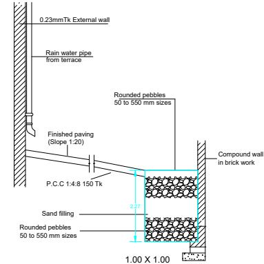
PLAN OF RAIN WATER HARVESTING
