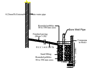
PLAN OF RAIN WATER HARVESTING
