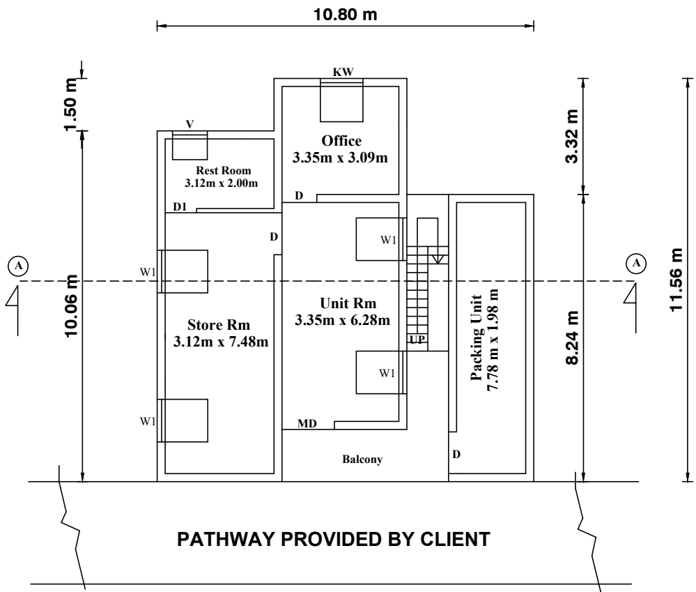
EXISTING GROUND FLOOR PLAN ( NORTH FACING )
