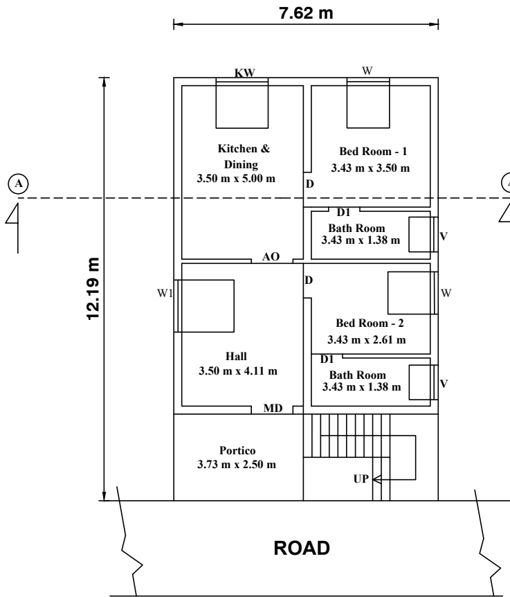
PROPOSED GROUND FLOOR PLAN NORTH FACING
