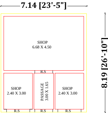
FIRST FLOOR PLAN WEST FACING
