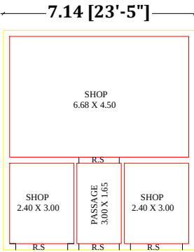
GROUND FLOOR PLAN WEST FACING
