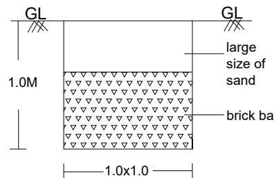
RAINWATER HARVESTING
