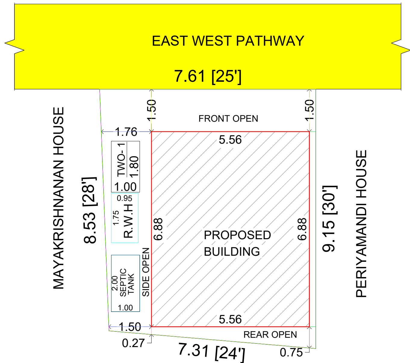
SELVARAJ-BOTHARAJ HOUSE COMMON PATHWAY
