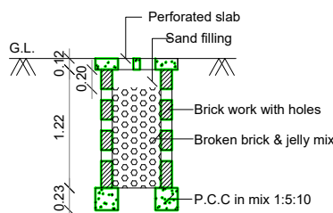
PERCOLATION PIT
