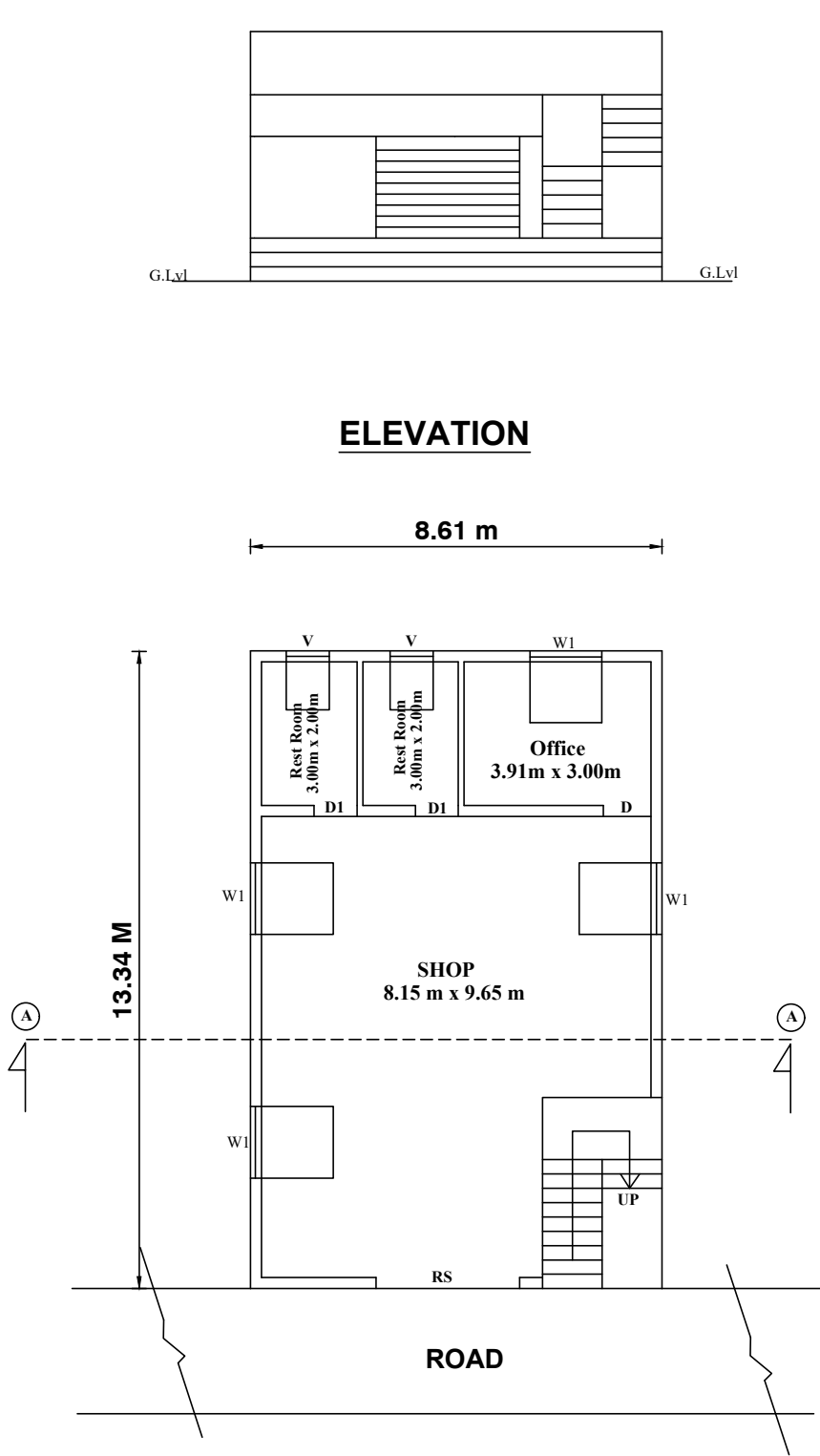
PROPOSED GROUND FLOOR PLAN ( SOUTH FACING)
