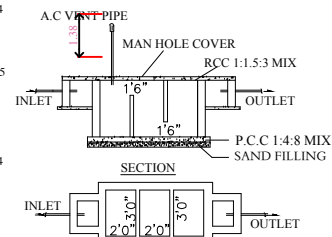
PLAN DETAILS OF SEPTIC TANK (Not to scale)
