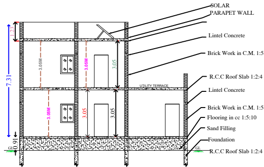
Sectional Details on AA'
