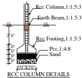
RCC COLUMN DETAILS
