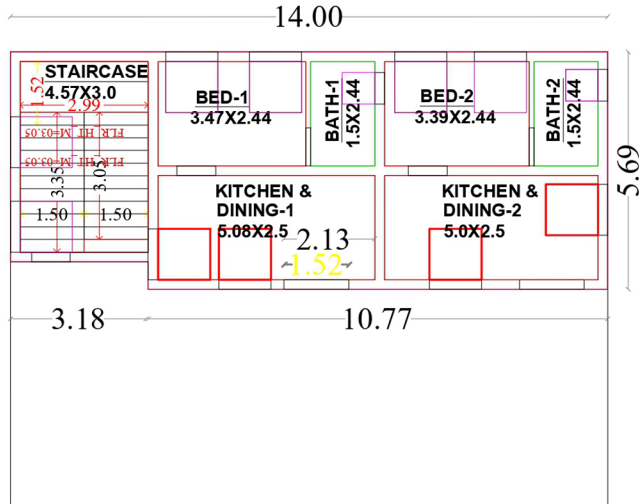
FIRST FLOOR PLAN (FACEING OF EAST)
