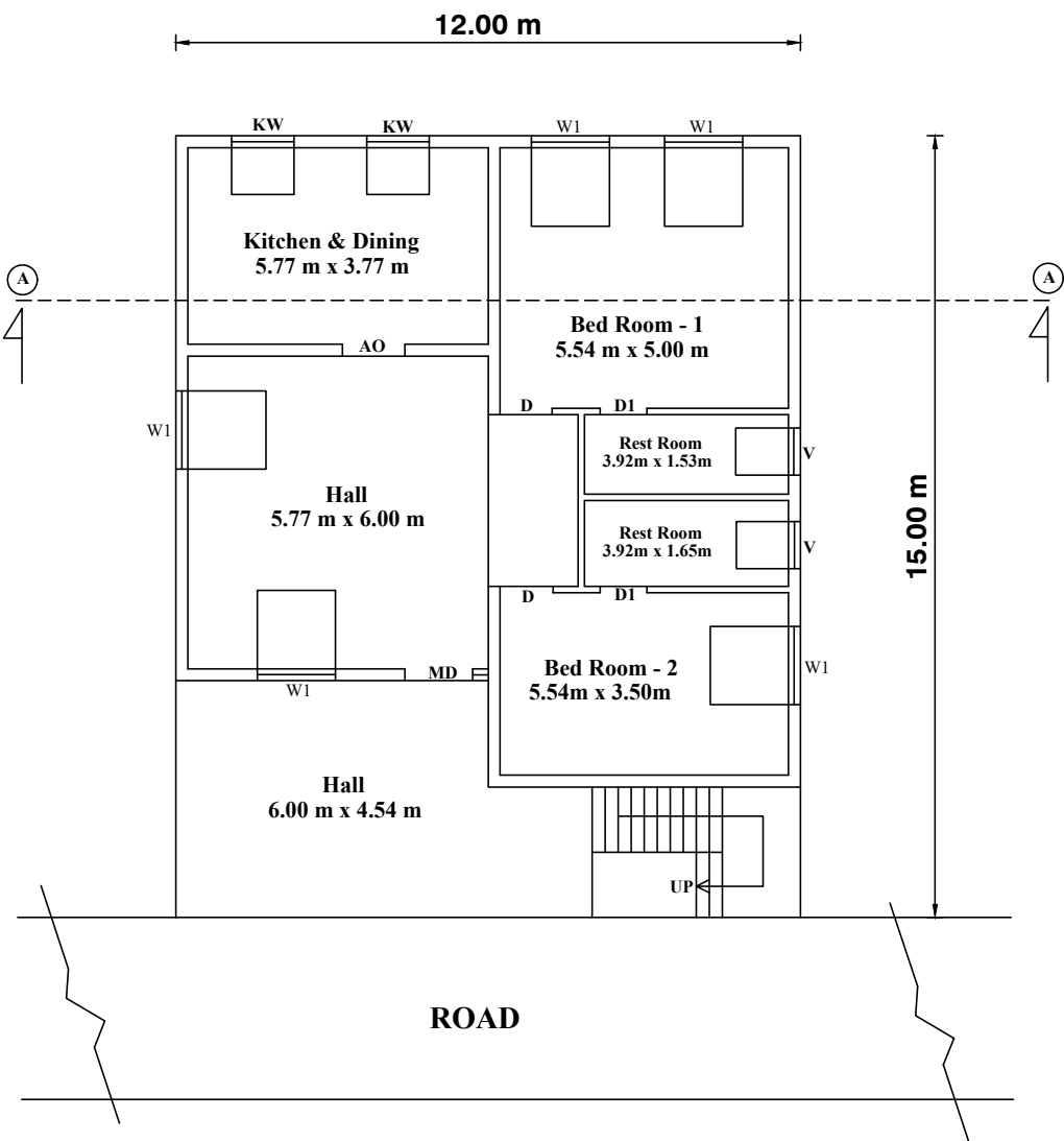
PROPOSED GROUND FLOOR PLAN ( NORTH FACING )
