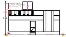
FRONT ELEVATION (EAST FACING)
