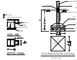
FOUNDATION DETAIL (SCALE 1:50)
