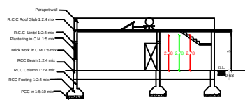
SECTION ON 'AA'
