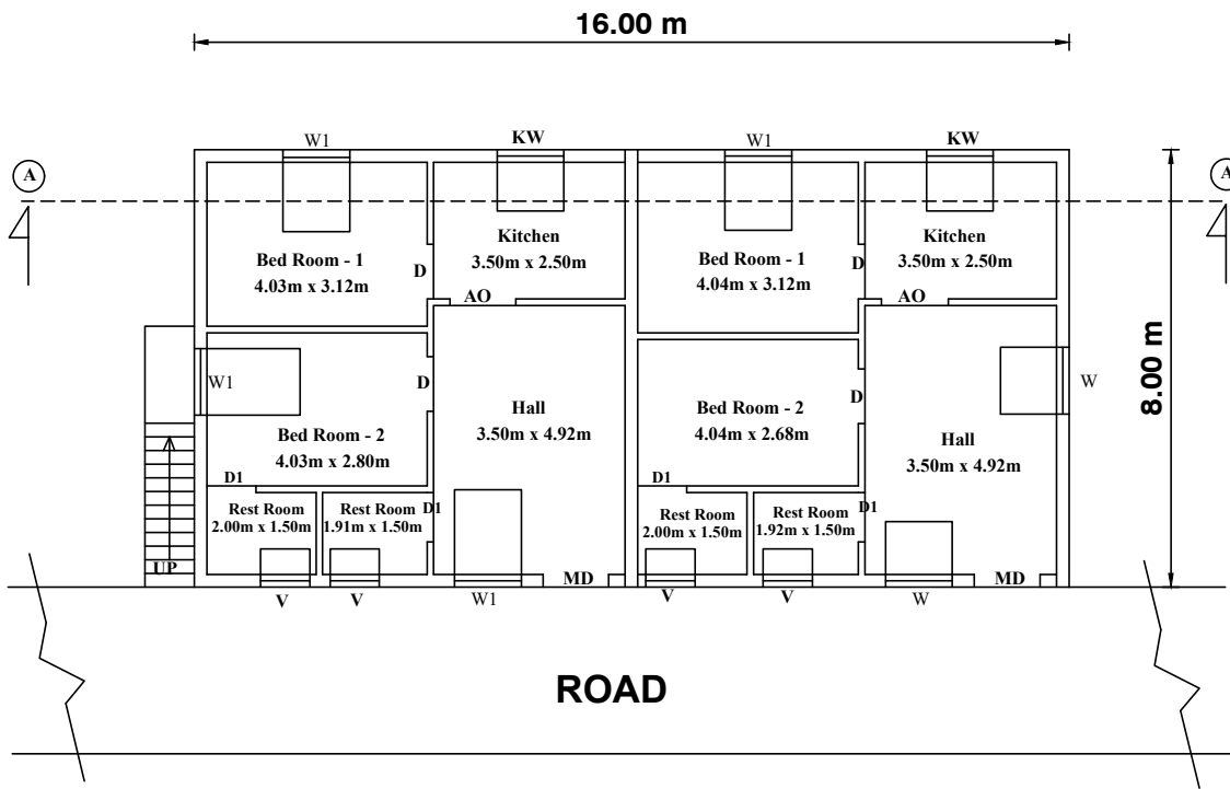
EXISTING GROUND FLOOR PLAN ( WEST FACING)
