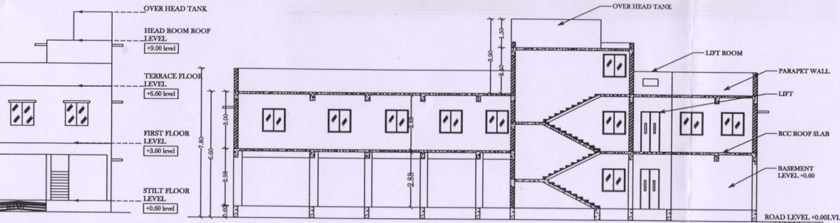
FRONT ELEVATION SECTION A-A
