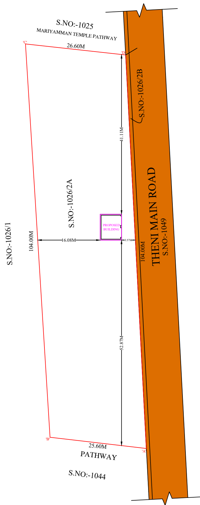
SITE PLAN
