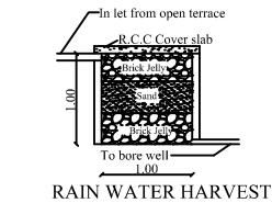
RAIN WATER HARVEST
