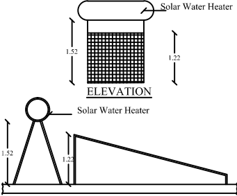
SECTION SOLAR WATER HEATER DETAILS
