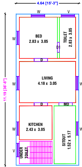
GROUND FLOOR PLAN [ EAST FACING ]
