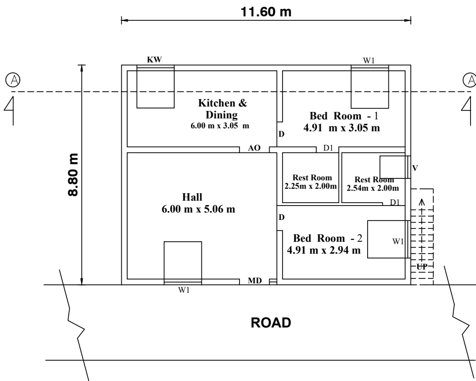
PROPOSED GROUND FLOOR PLAN ( NORTH FACING )
