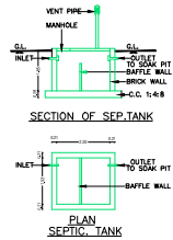
SECTION OF SEPTIC TANK
