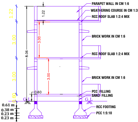
SCETION ON A-A
