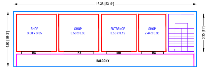
GROUND FLOOR PLAN [ NORTH FACING ]
