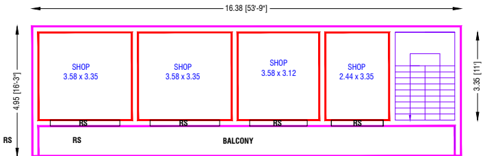
FIRST FLOOR PLAN [ NORTH FACING ]
