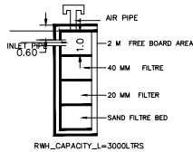
AIR PIPE 2 M FREE BOARD AREA 40 MM FILTER 20 MM FILTER SAND FILTER BED RWHD_CAPACITY_L=3000LTRS
