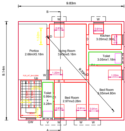
GROUND FLOOR PLAN [WEST FACING]
