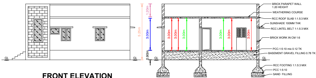
CROSS SECTION - 'AB'
