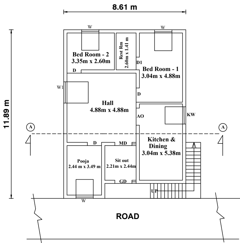
EXISTING GROUND FLOOR PLAN SOUTH FACING
