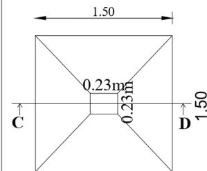
SECTION - 'CD' FOUNDATION DETAIL - A
