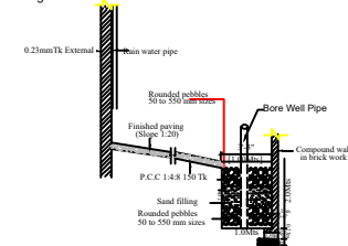
PLAN OF RAIN WATER HARVESTING
