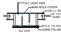
PLAN DETAILS OF SEPTIC TANK (Not to scale)
