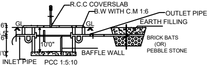
SEPTIC TANK DETAILS
