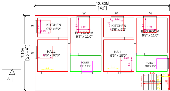
PRO.GROUND FLOOR PLAN
