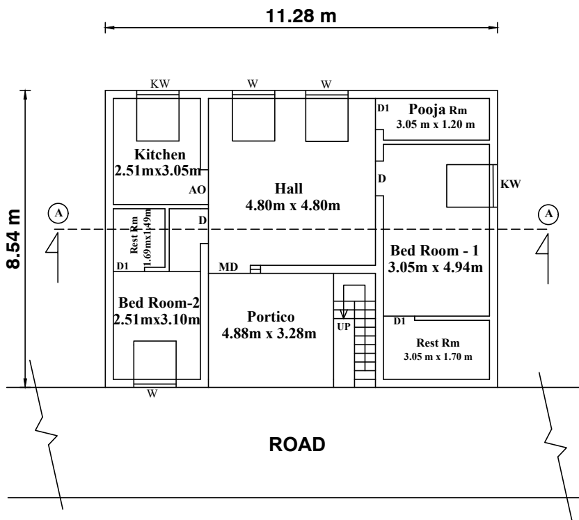
EXISTING GROUND FLOOR PLAN NORTH FACING
