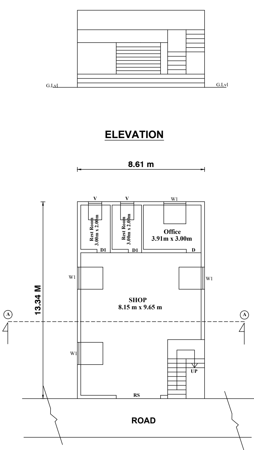
PROPOSED GROUND FLOOR PLAN ( SOUTH FACING - EAST BLOCK)
