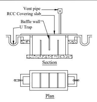
Using 'U' type trap 2 Nos in inlet, outlet & Ventpipe will be covered with mosquito proof covering net in inner side of vent pipe and top of vent pipe
