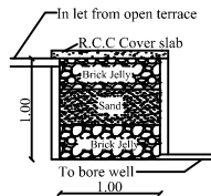
RAIN WATER HARVEST
