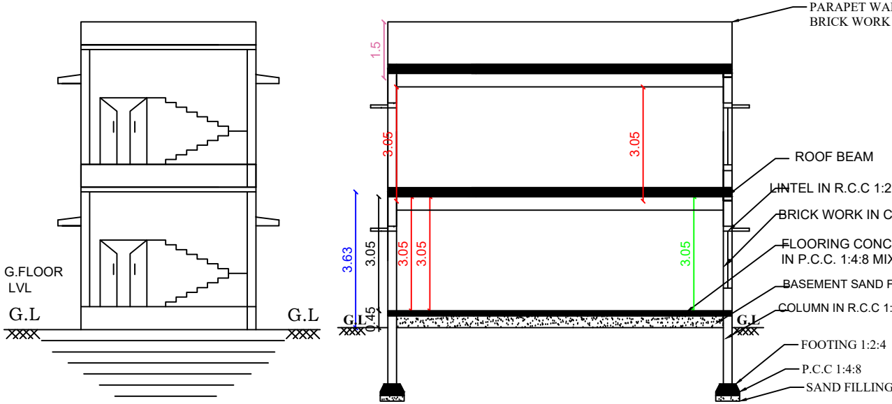
ELEVATION (North Facing)
