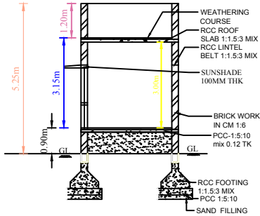
CROSS SECTION - 'AB'
