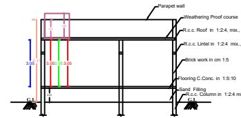
SECTION ON "AA"
