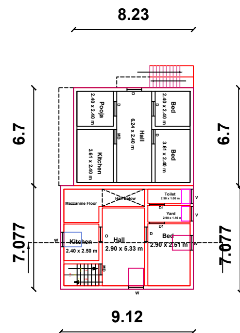
EXISTING FIRST FLOOR PLAN ( SOUTH FACING ) PROPOSED FIRST FLOOR PLAN ( EAST FACING )
