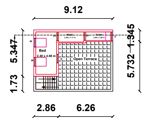
PROPOSED SECOND FLOOR PLAN & TERRACE FLOOR PLAN
