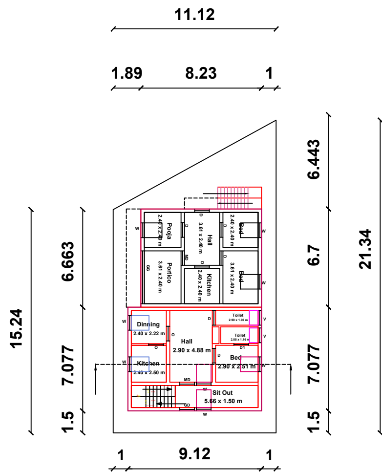
SOUTH FACING ( EAST FACING )
