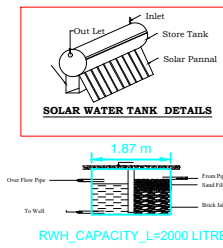
RWH_CAPACITY_L=2000 LITRE
