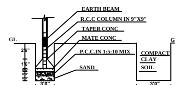
FOUNDATION DETAILS
