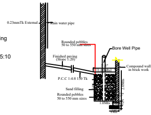
PLAN OF RAIN WATER HARVESTING
