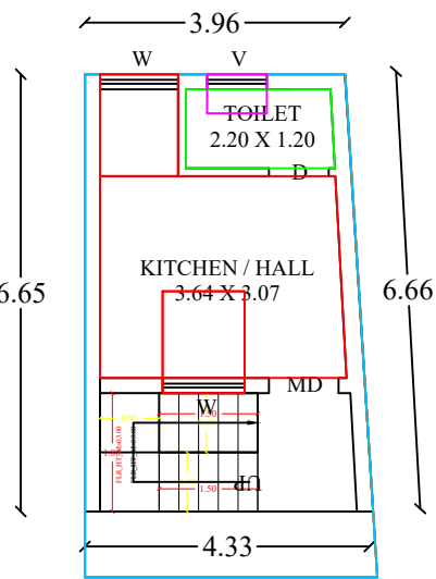
GROUND FLOOR PLAN (EAST FACING)
