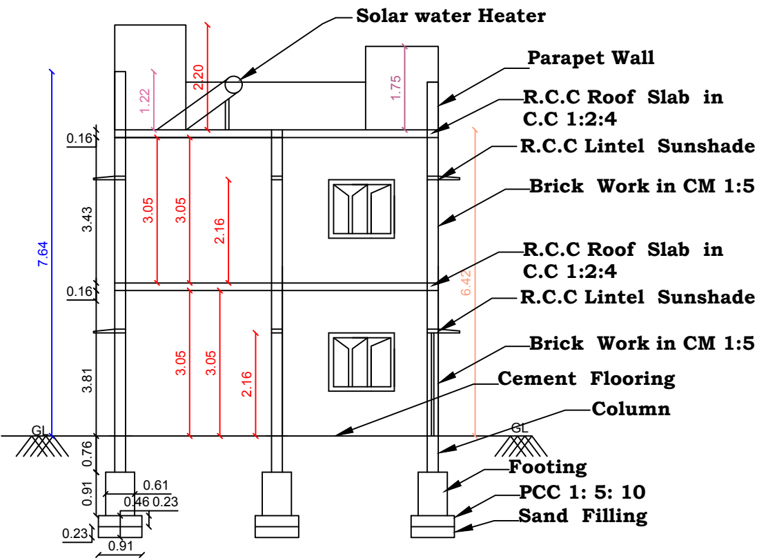
SECTION - BB
