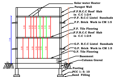
Sectional View
