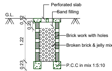
PERCOLATION PIT
