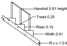
STAIECASE DETAILS
