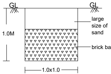
RAINWATER HARVESTING
