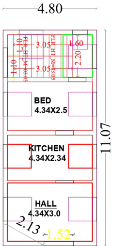
GROUND FLOOR PLAN (FACING OF WEST)
