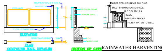
RAINWATER HARVESTING
