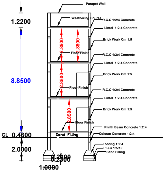
Section Section - AA
