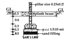
FOUNDATION DETAILS
