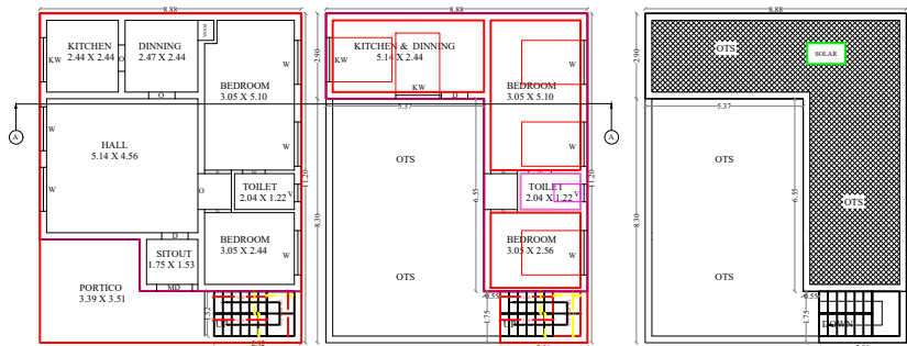
EXISTING GROUND FLOOR PLAN (NORTH FACING)
