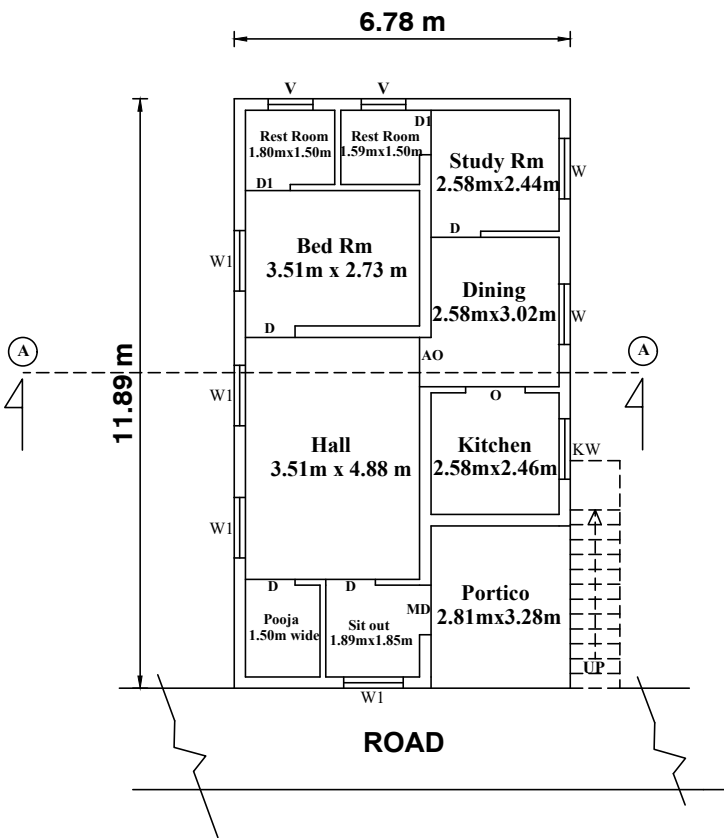
EX. GROUND FLOOR PLAN
