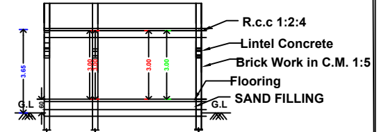
SECTION ON "BB"
