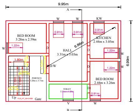
GROUND FLOOR PLAN (WEST FACING)
