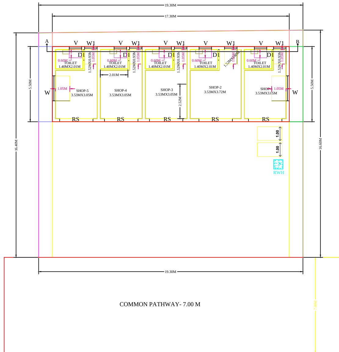
BLOCK-1 GROUND FLOOR PLAN
