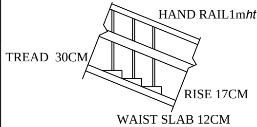
STAIRCASE DETAILS
