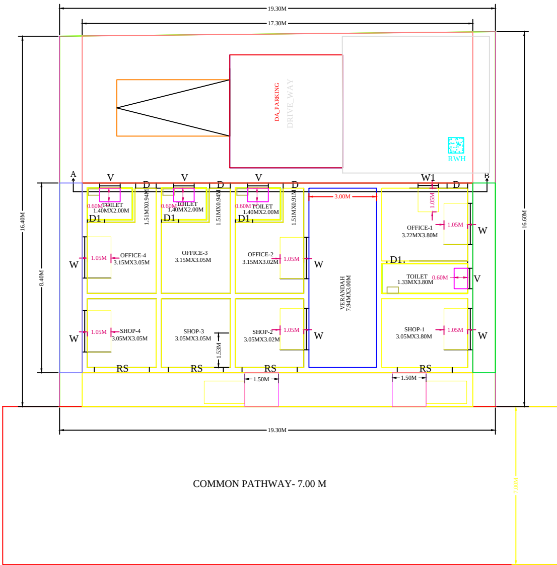
BLOCK-2 GROUND FLOOR PLAN
