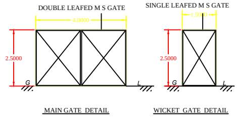
MAIN GATE DETAIL
