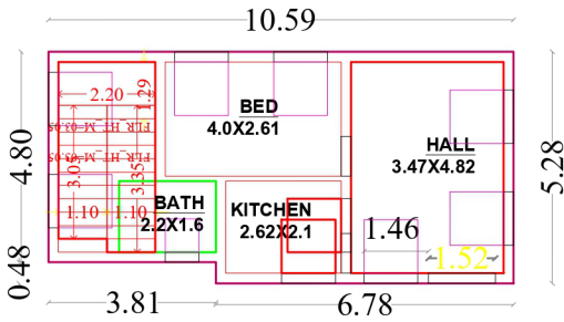
GROUND FLOOR PLAN (FACEING OF SOUTH)
