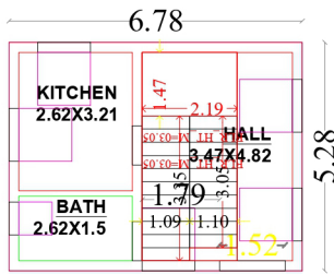
FIRST FLOOR PLAN (FACEING OF SOUTH)
